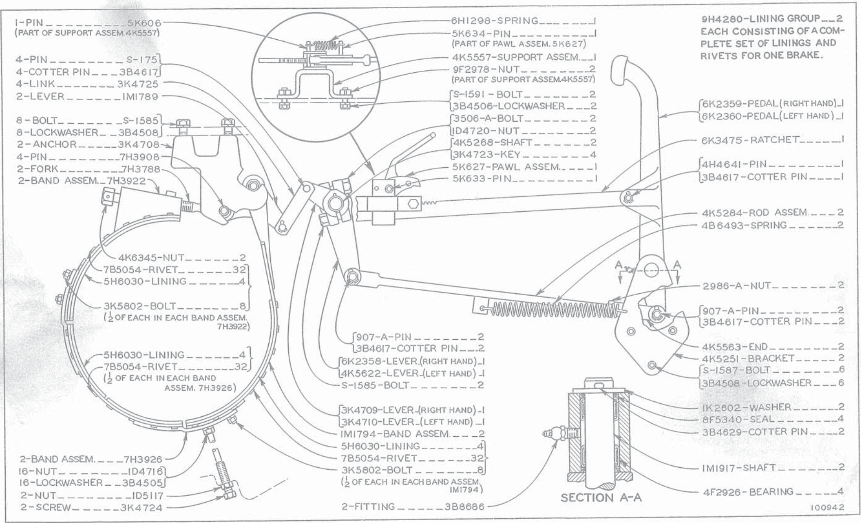
BRAKES (6K2380 N/S) Serial No. 83J1 to 83J1268 inclusive
